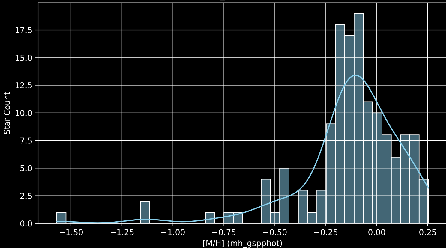
APOGEE DR17 Field: [188-12 [M/H] (mh_gspphot) (n= 141)
