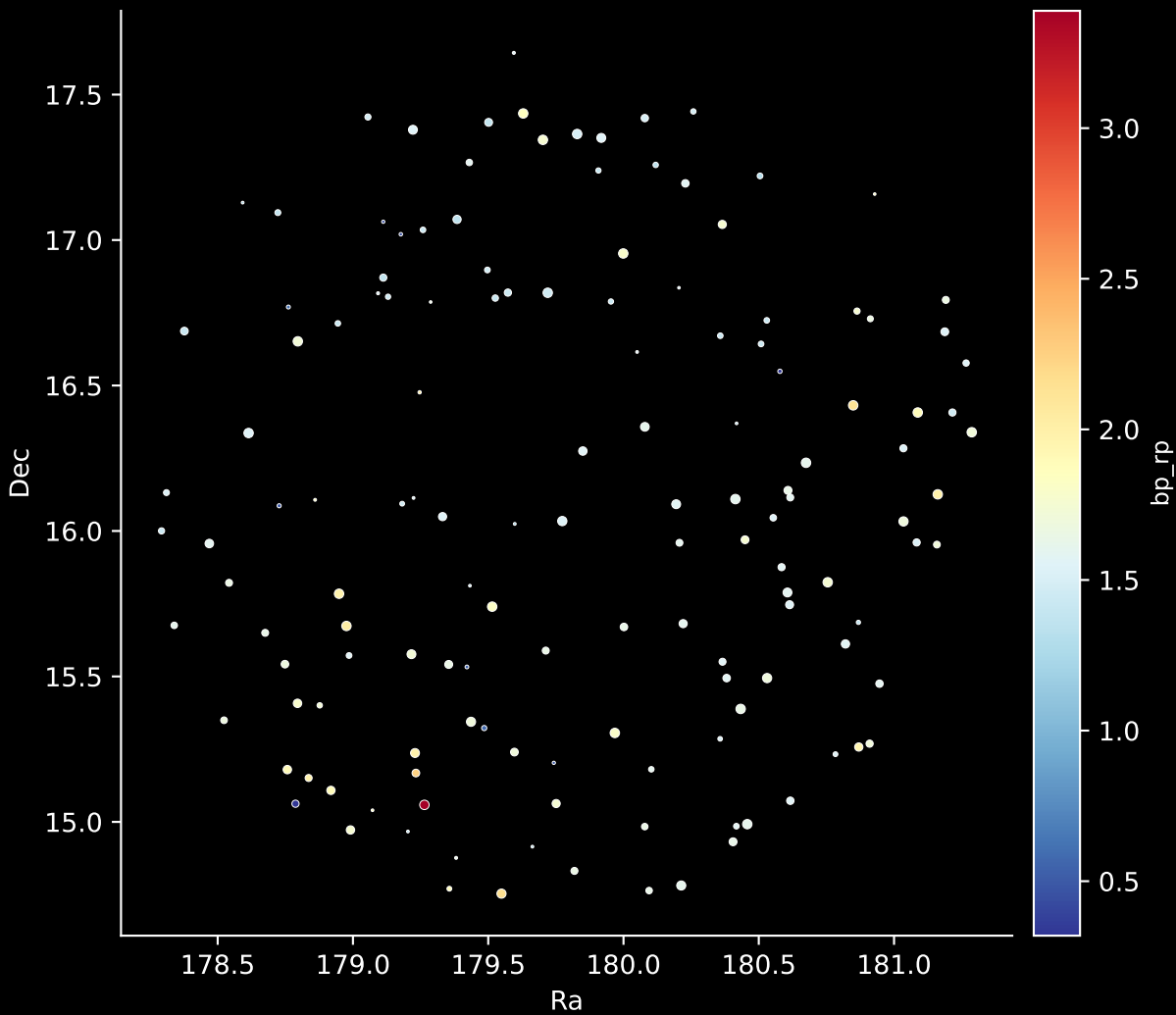
APOGEE DR17 Field: [188-12] Stars: 142
