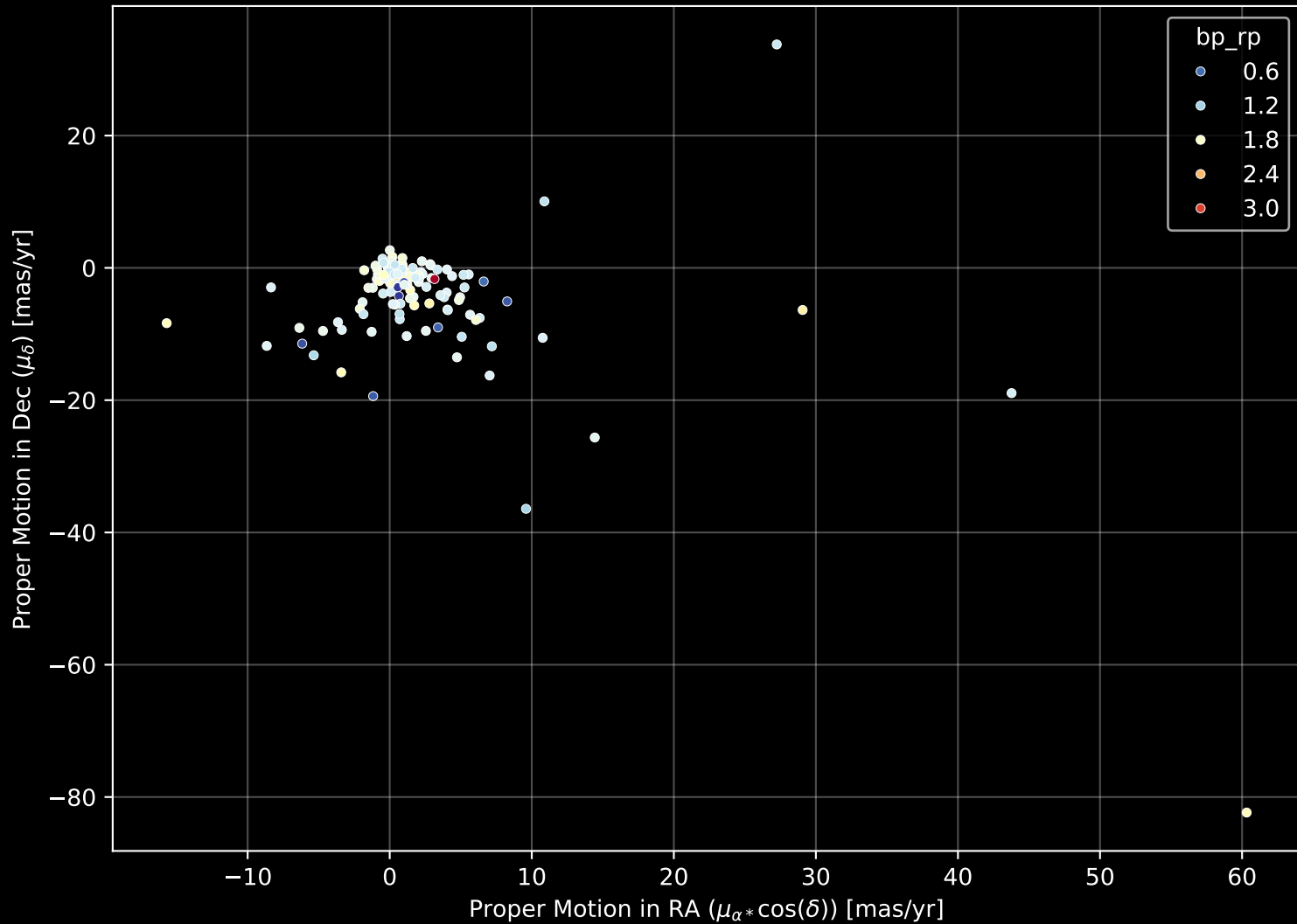
APOGEE DR17 Field: [188-12] Proper Motion Diagram (n= 142)
