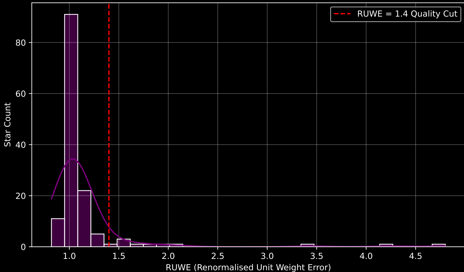
GAPOGEE DR17 Field [188-12] RUWE Distribution (n= 140)
