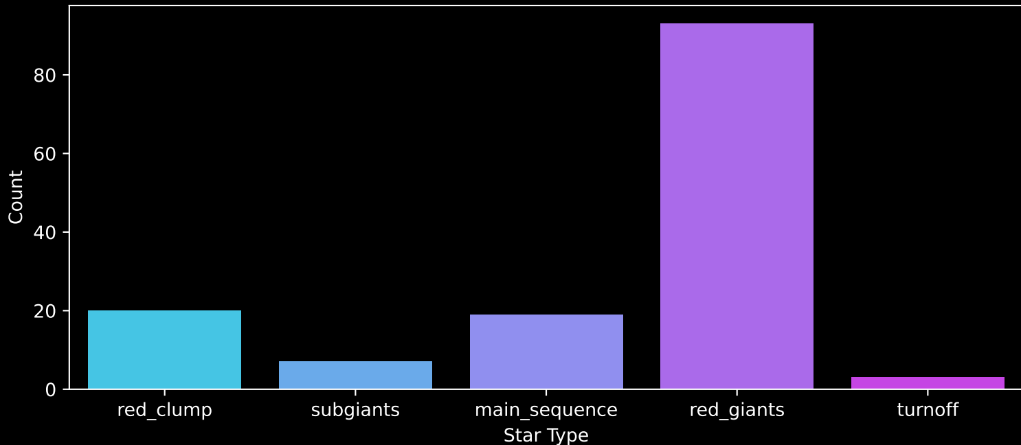
APOGEE DR17 Field: [188-12] Count plot of Star Type
