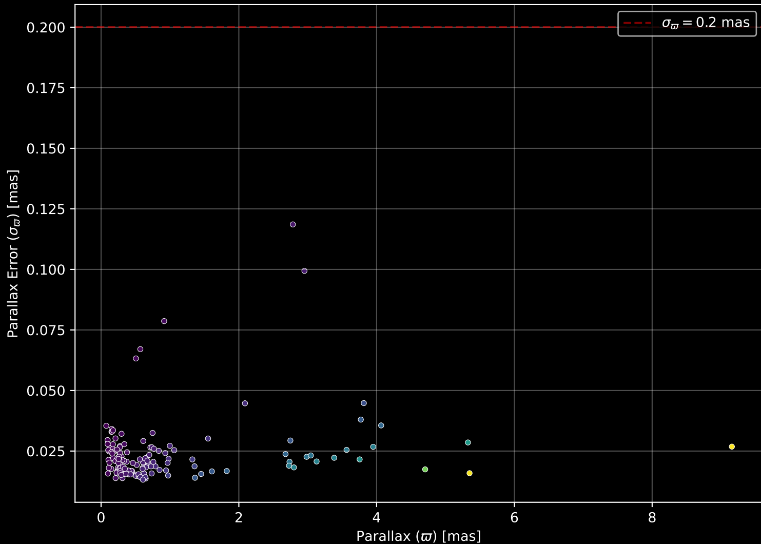
APOGEE DR17 Field: [188-12] Parallax Quality (n= 142)
