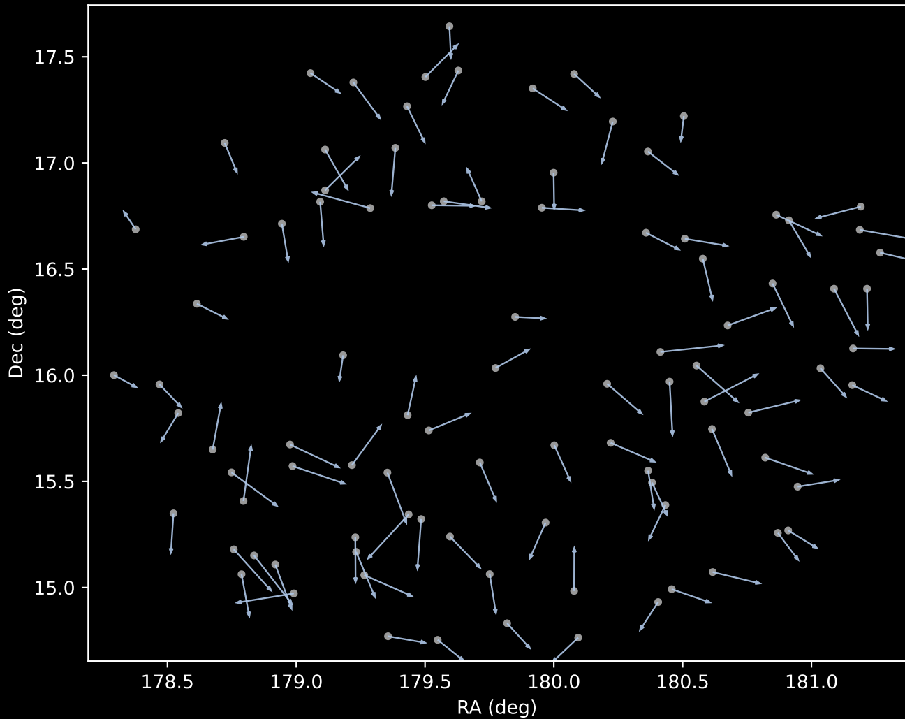
APOGEE DR17 Cluster 1 Proper Motion Vectors (n=95)
